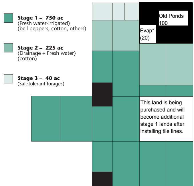
Figure 2. AndrewsAg IFDM. Sequential reuse, 3 stages (1035 acres).
